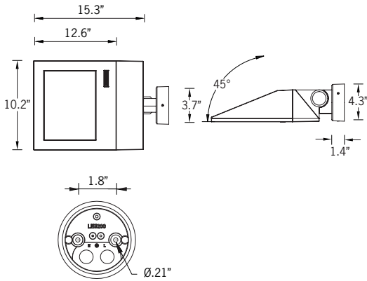
Mounting Detail
