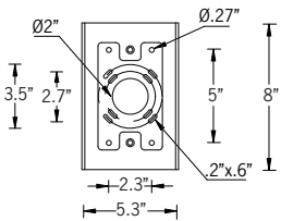
Mounting Detail
