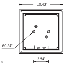
Mounting Detail
