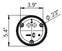
Mounting Detail
