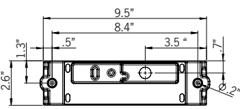
Mounting Detail
