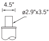
Tenon Detail
