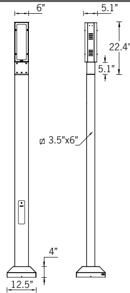
Mounting Detail
