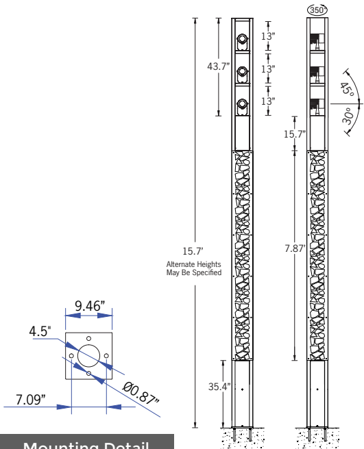
Mounting Detail
