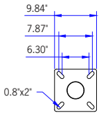
Mounting Detail
