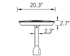
Fixture Detail
