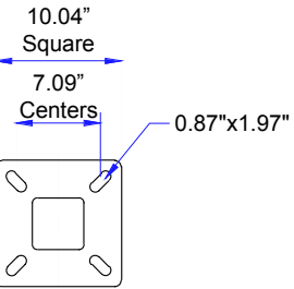
Mounting Detail
