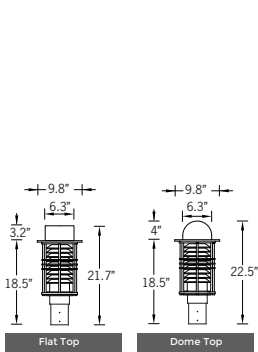
Lantern Detail
