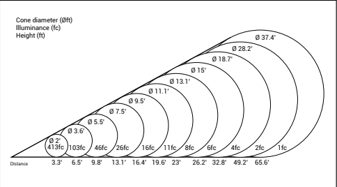
ODESSA 2-G (Wide)
