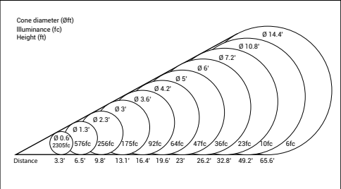
ODESSA 2-G (Narrow)
