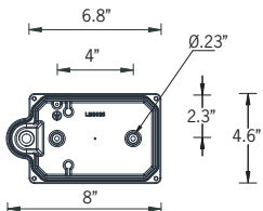
Mounting Detail
