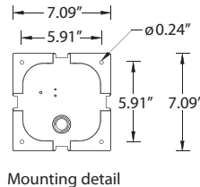
Mounting detail
