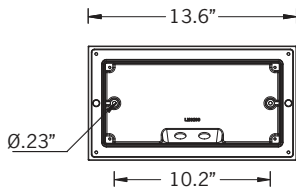
Mounting Detail
