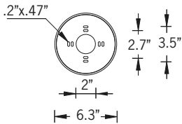
Mounting Detail
