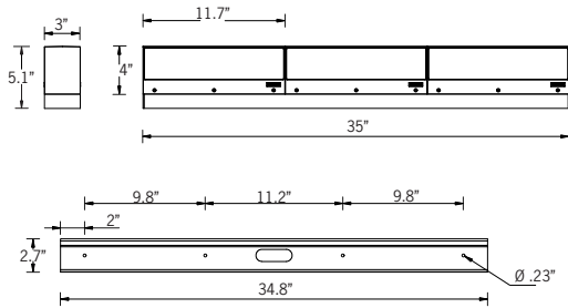
Mounting Detail
