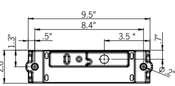
Mounting Detail
