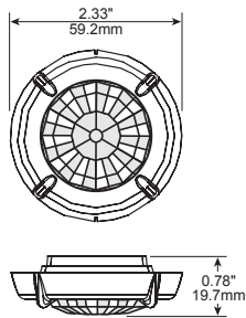
FSP-L3 dimensions
