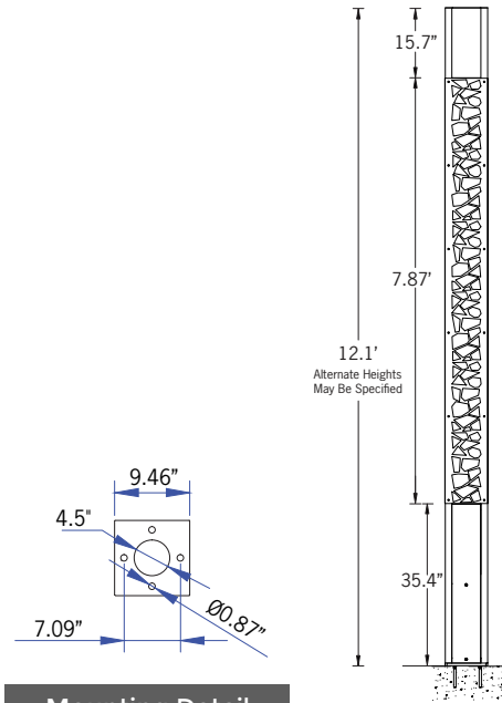
Mounting Detail
