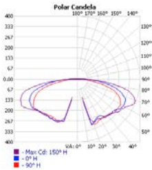
134° Beam Spread
