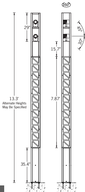
Mounting Detail
