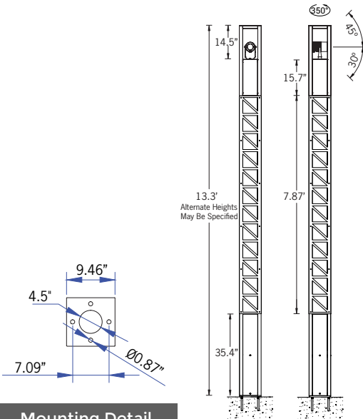
Mounting Detail
