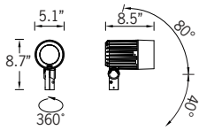
Floodlight Detail
