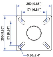
Mounting Detail
