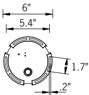
Mounting Detail
