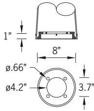
Mounting Detail
