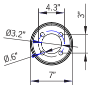
Mounting Detail
