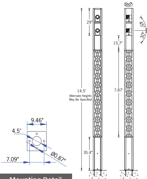
Mounting Detail
