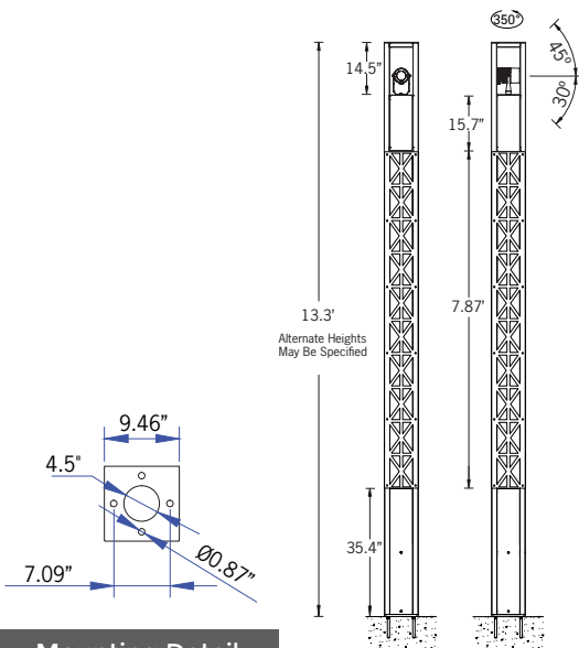
Mounting Detail
