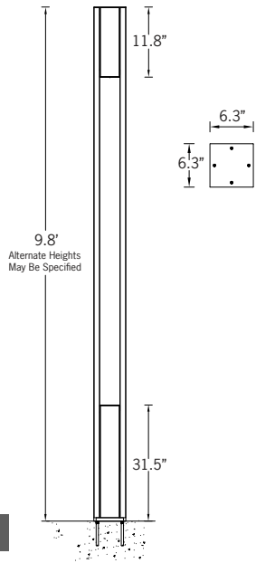
Mounting Detail
