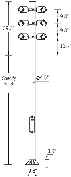
Mounting Detail
