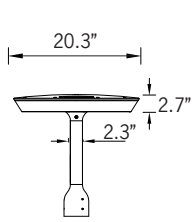
Fixture Detail
