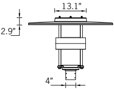
Fixture Detail
